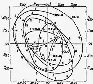
Fig. 13. Wandering of the pole from 1890 to 1898.
